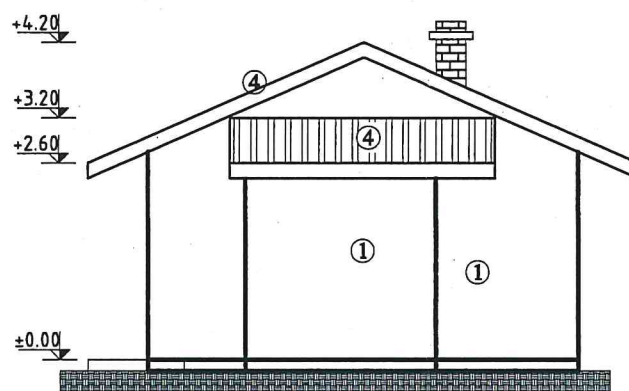
FATADA LATERALA D - D
