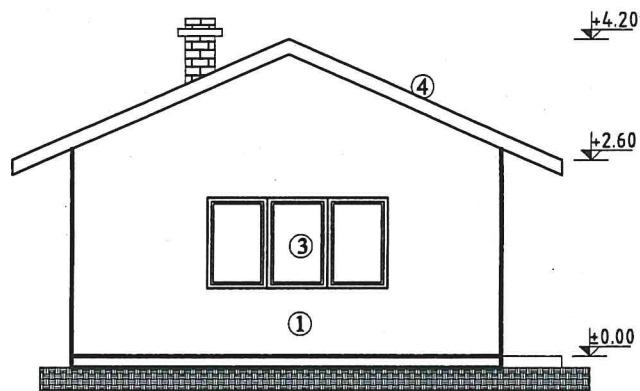
FATADA LATERALA B - B
